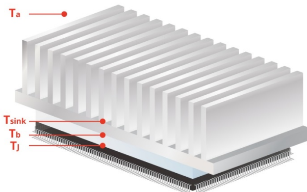
▲ Thermal module temperature description of flat type heat sink
