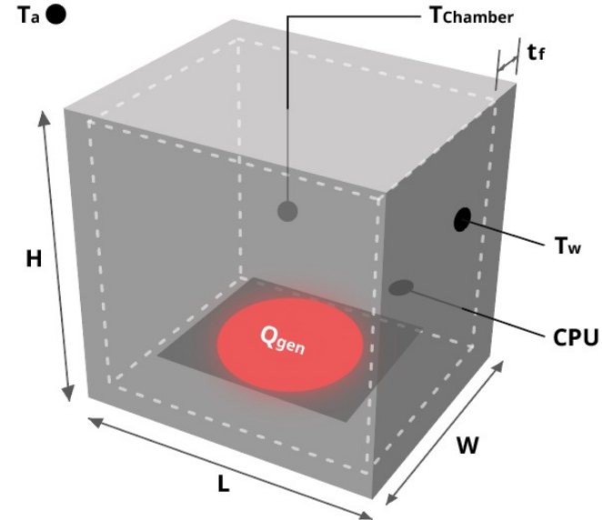
▲ Schematic diagram of chamber
